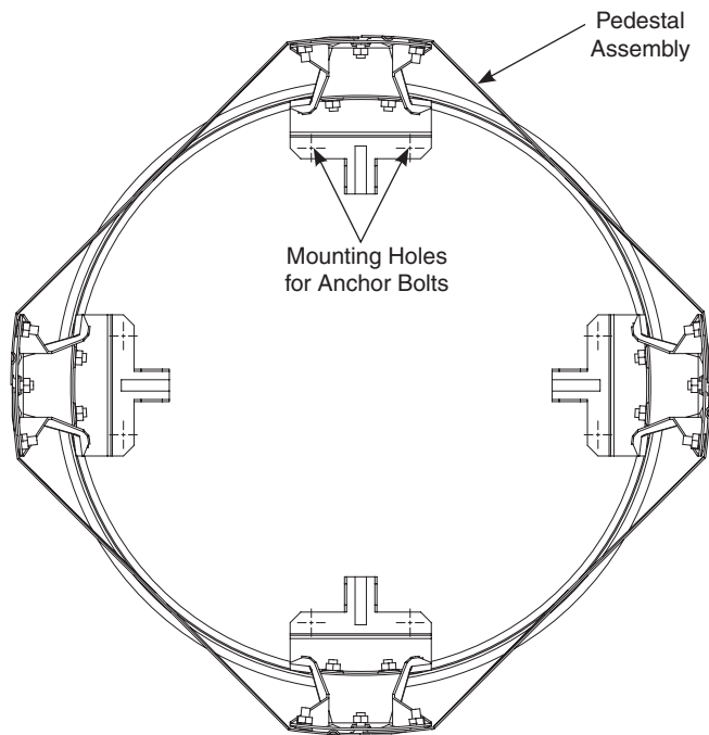
TOP VIEW OF PEDESTAL ASSEMBLY
