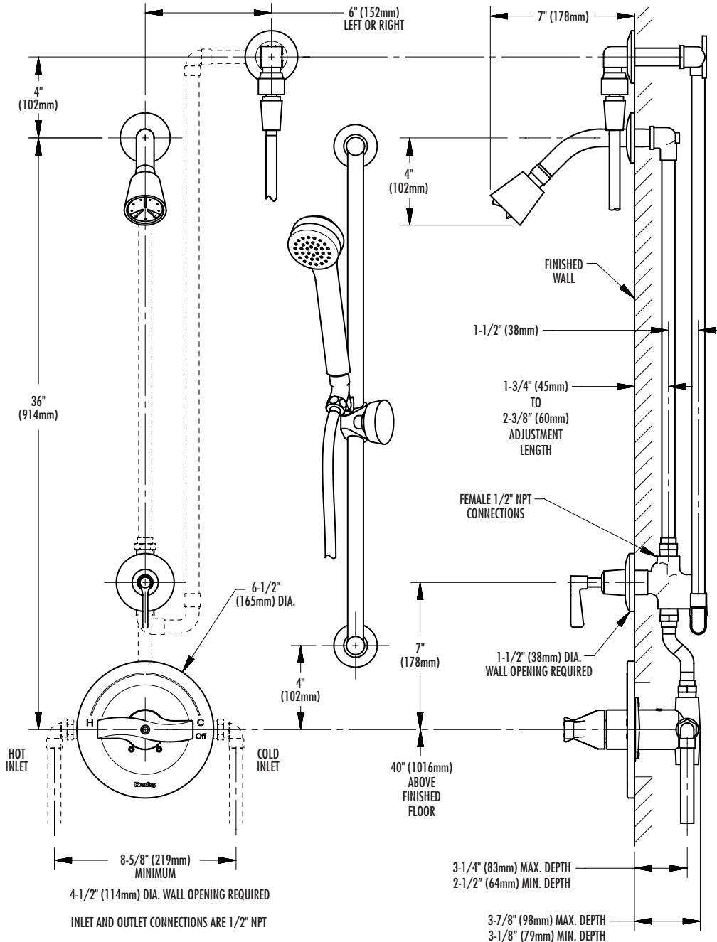
HAND SHOWER AND SHOWERHEAD
